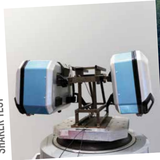
WEATHERING TEST
