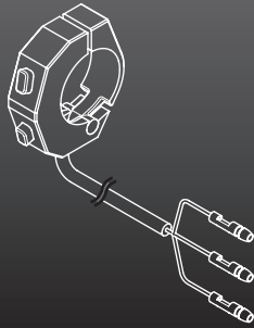
Wiring outside handle bar
